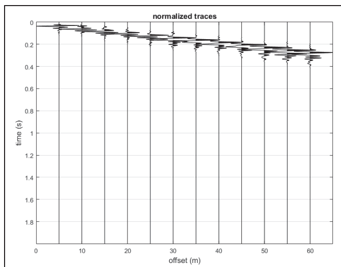
Figura 9: Sismogramma ZVF (onde Rayleigh) base sismica L1.
